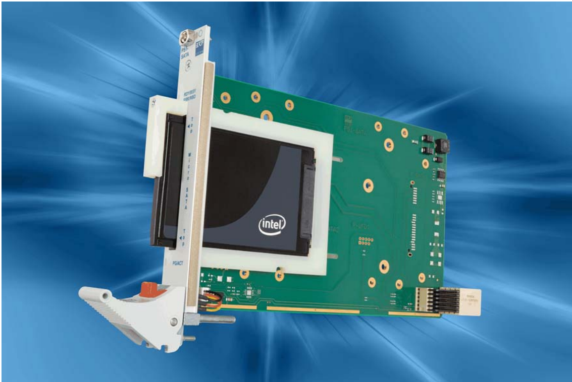
PS1-SATA with Front Panel Removable SSD
